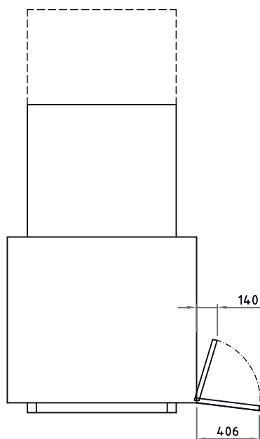
Vista frontal
